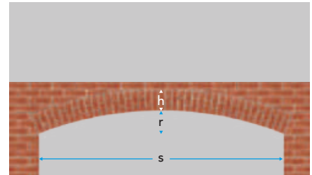
Front elevation notes the essential measurements required to specify the Segmental Arch BFL.
