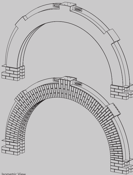
Isometric View
