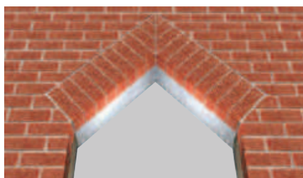
View showing the underside of Keystone's Apex BFL. This illustrates how the brickwork returns under the soffit of the lintel to ensure no steelwork is visible on the outer leaf.
