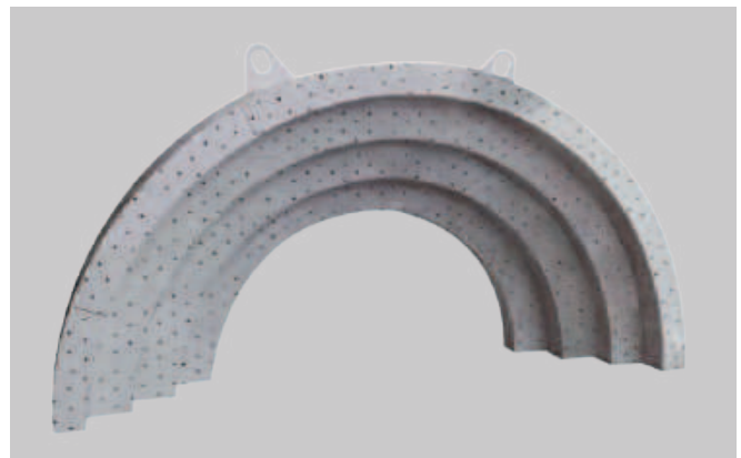
Corbelled Arch Brick Feature Lintel frame before cut bricks are attached.
