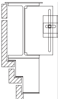
Section View
