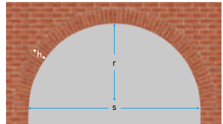
Front elevation notes the essential measurements required to specify the Semi Circular Arch BFL.
